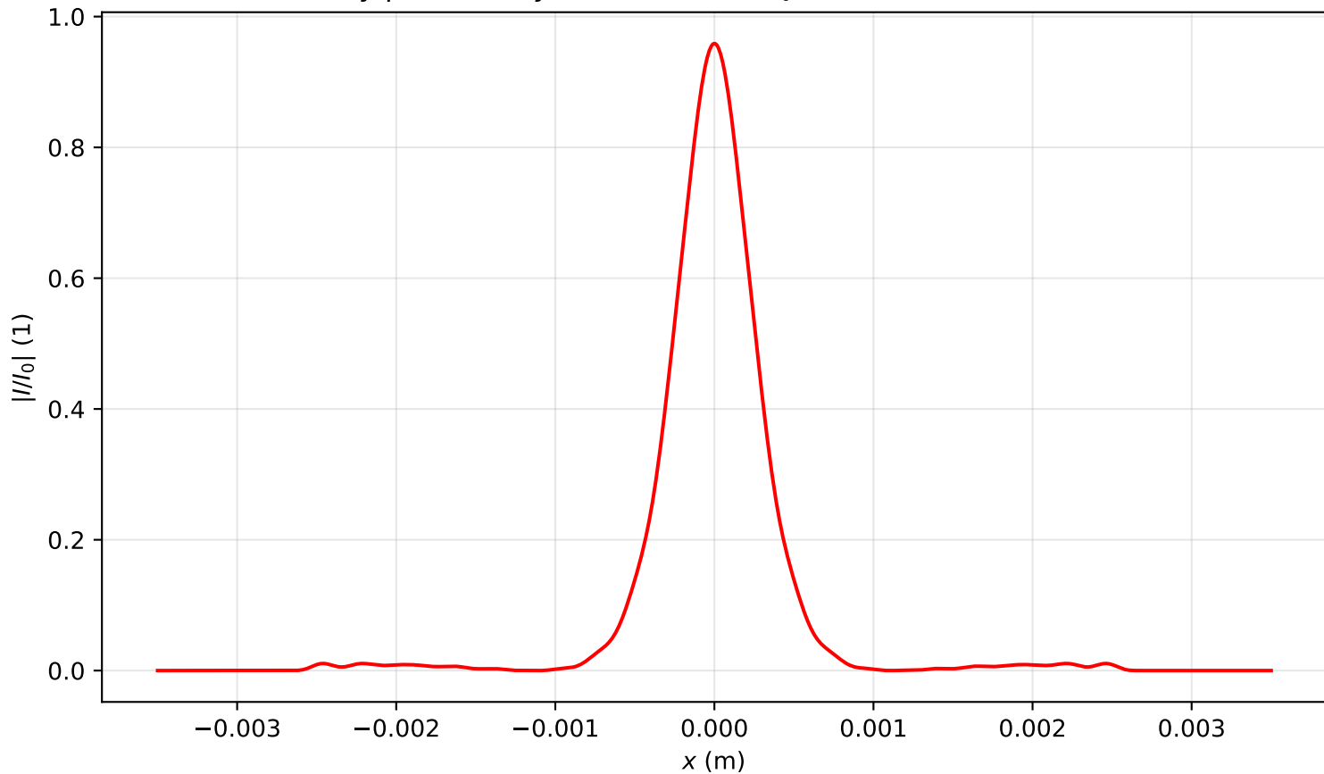
Intensity profile I(x, y = 0, z = 1.592)/I_0 , P_{in}=1.0P_{cr} , artificial time
